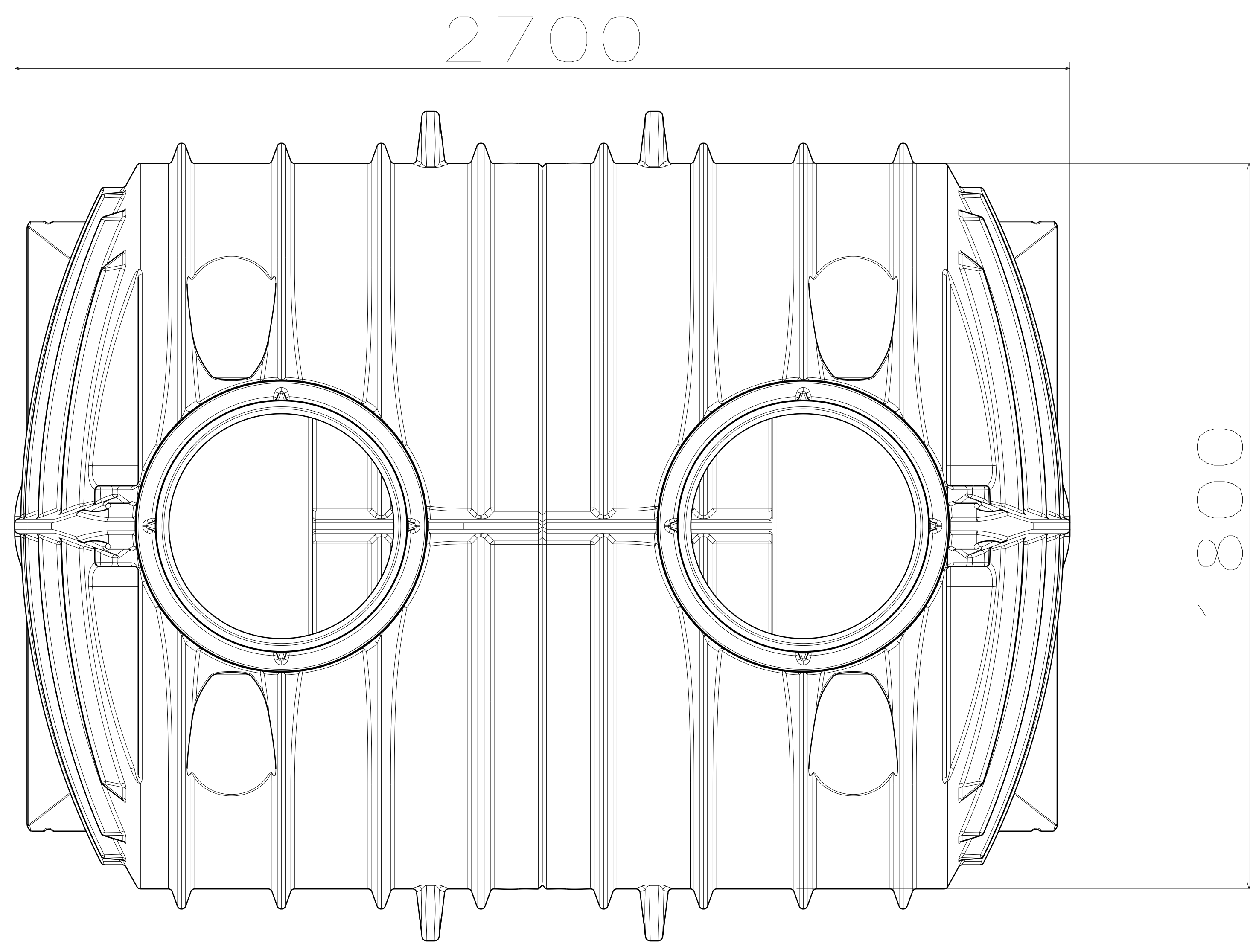
Front view Scale: 1:8
